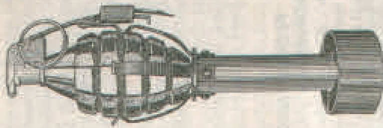
© Grenade-projection adapter M1, with hand grenade Mk. II.
