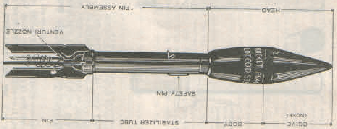
Figure 32. Primitive anti-air rocket, 2.56-inch, M241.
