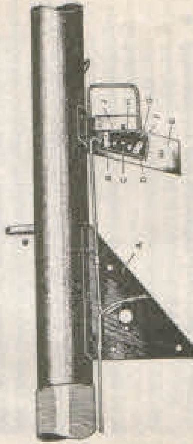
Figure 36. Trigger group, launcher M1A1.
