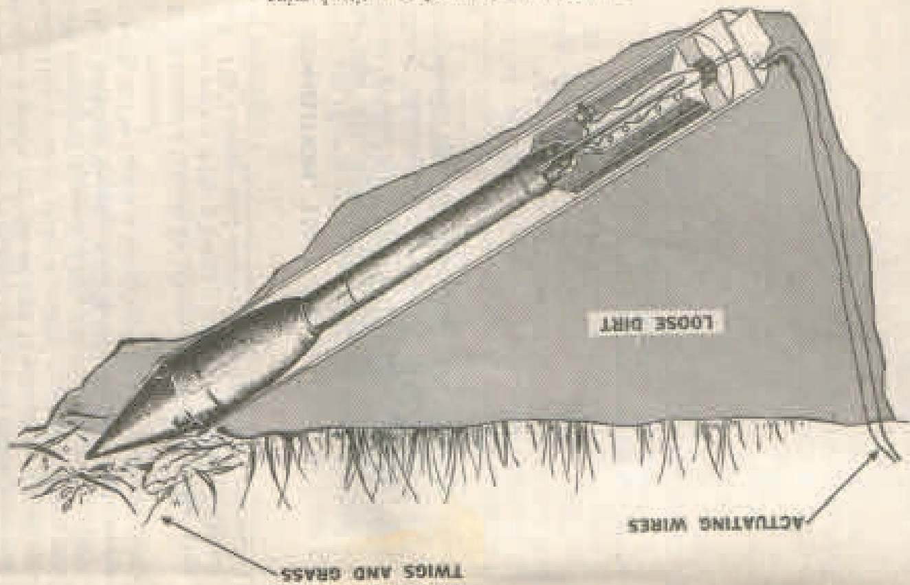
Figure 96. Rocket used as antitank mine.
